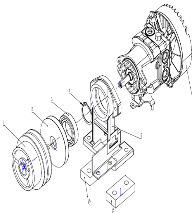
Engine output assembly
