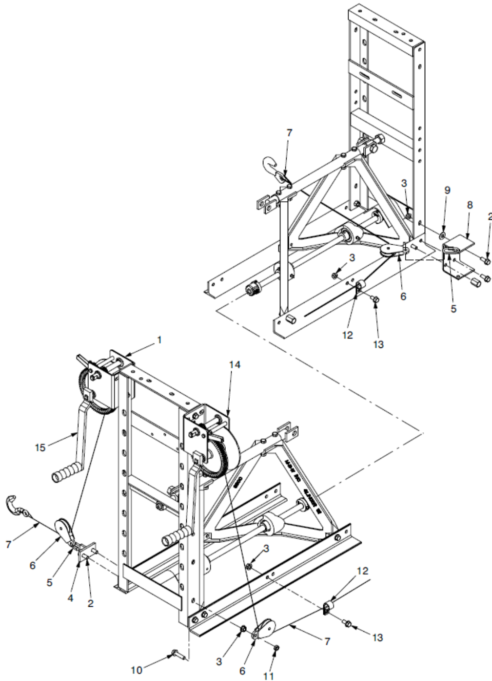
FIGURE 34: HAND WINCH KIT (Two winches One End)
