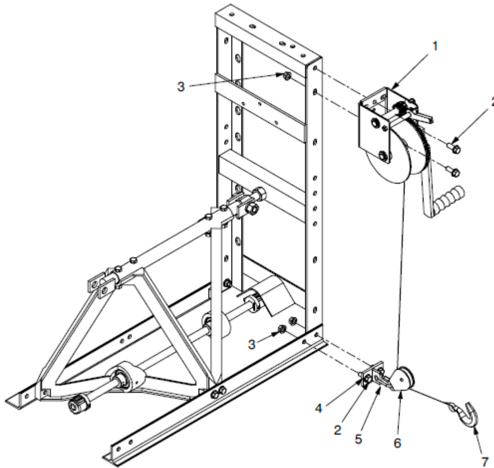
FIGURE 35: HAND WINCH KIT (One Winch Each end)
