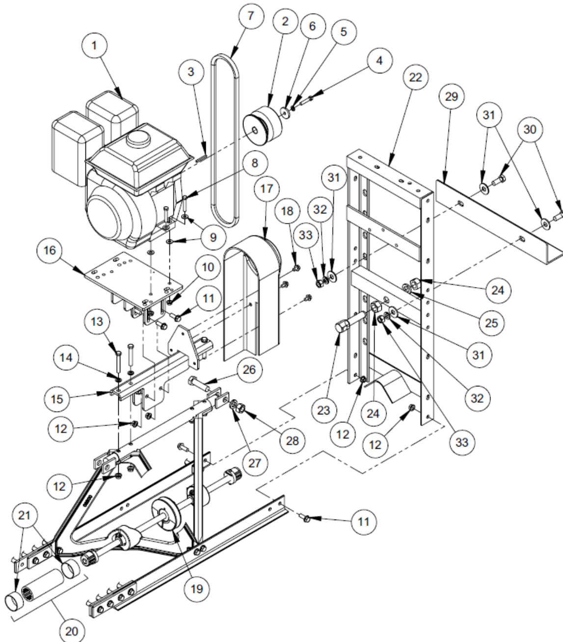
FIGURE 29: ENGINE KIT
