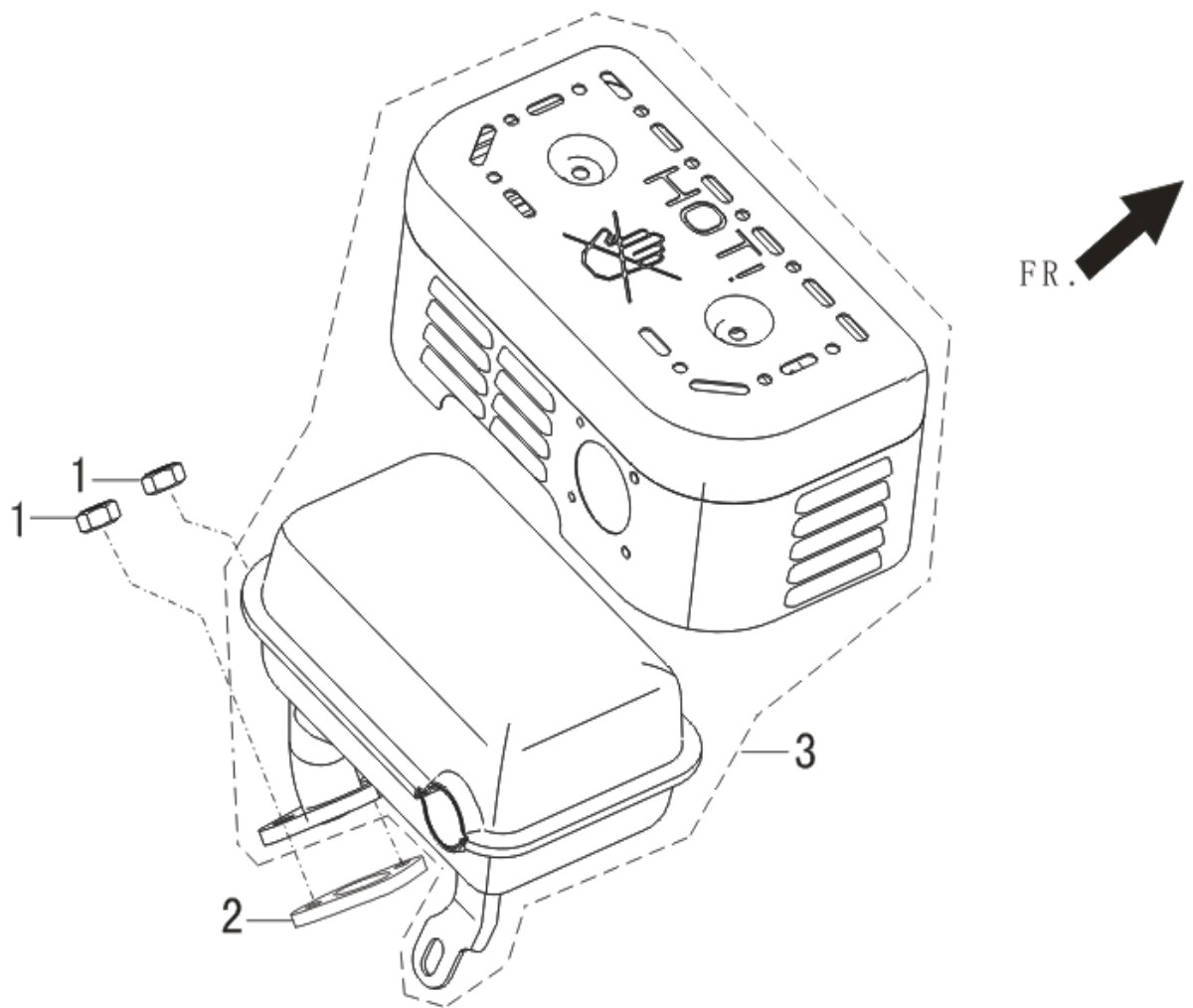
FIG.11 MUFFLER ASSY.
