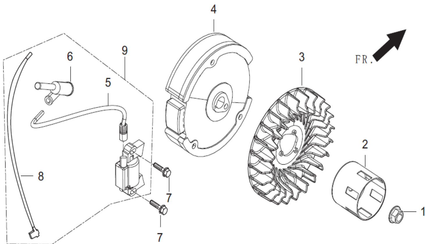
FIG.13 FLYWHEEL / IMPELLER / STARTER PULLEY / IGNITION COIL
