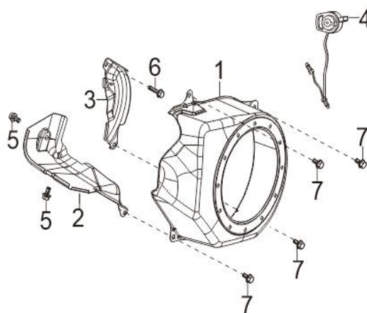
FIG.8 SHROUD / SHIELD,LOWER
