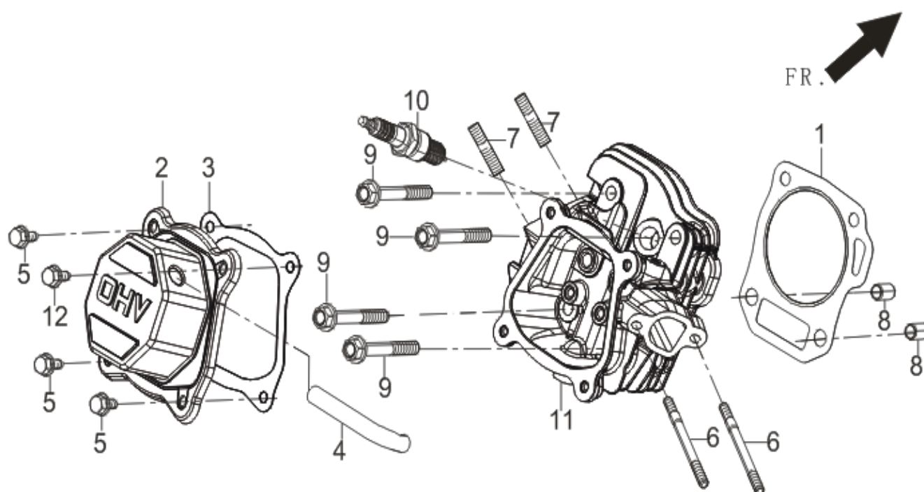
FIG.3 HEAD SUBASSEMBLY, CYLINDER / PLUG,SPARK
