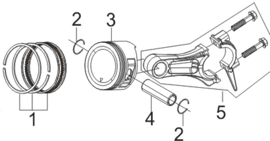
FIG.5 RING SET,OIL / ROD,CRANKSHAFT CONNETING
