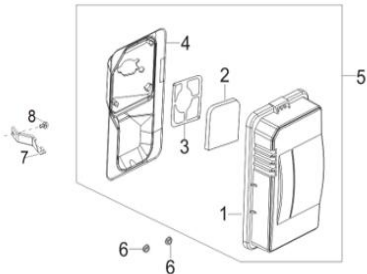
FIG.10 CLEANER, AIR
