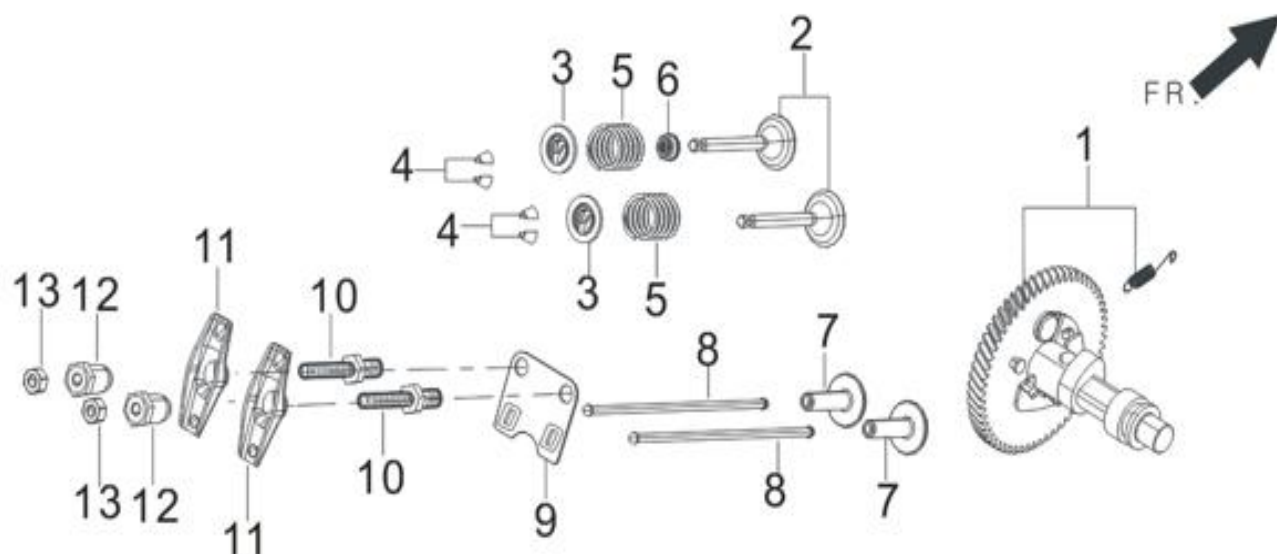
FIG.6 TRAIN,VALVE / CAMSHAFT SUBASSEMBLY
